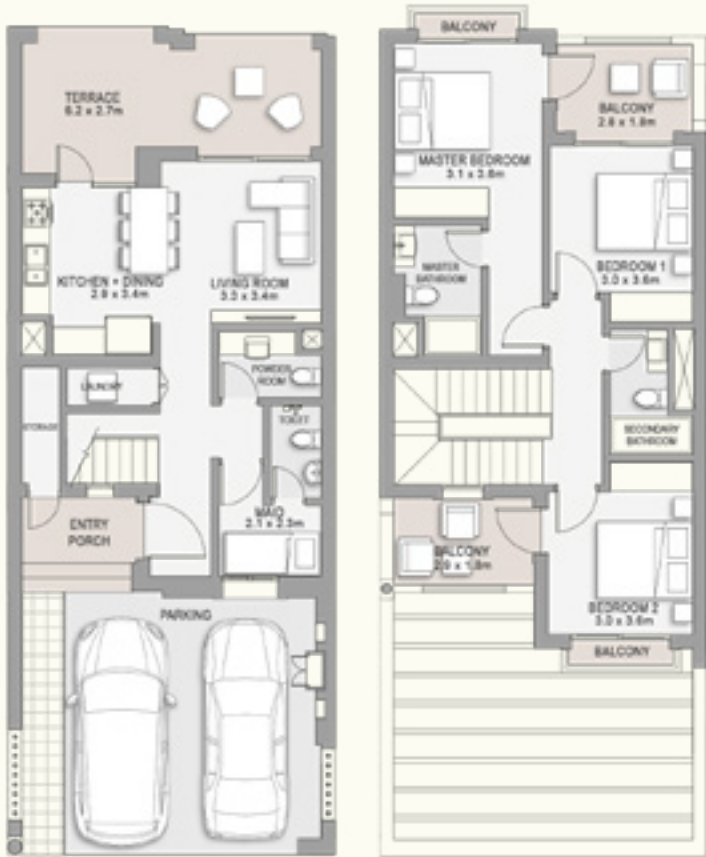
GROUND FLOOR FIRST FLOOR
