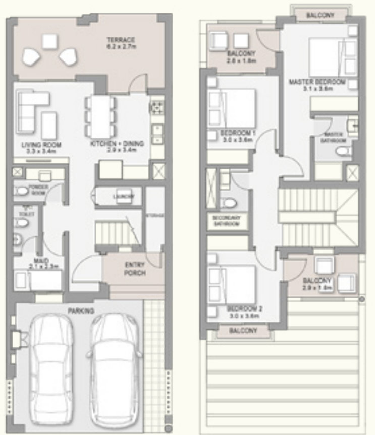
GROUND FLOOR FIRST FLOOR
